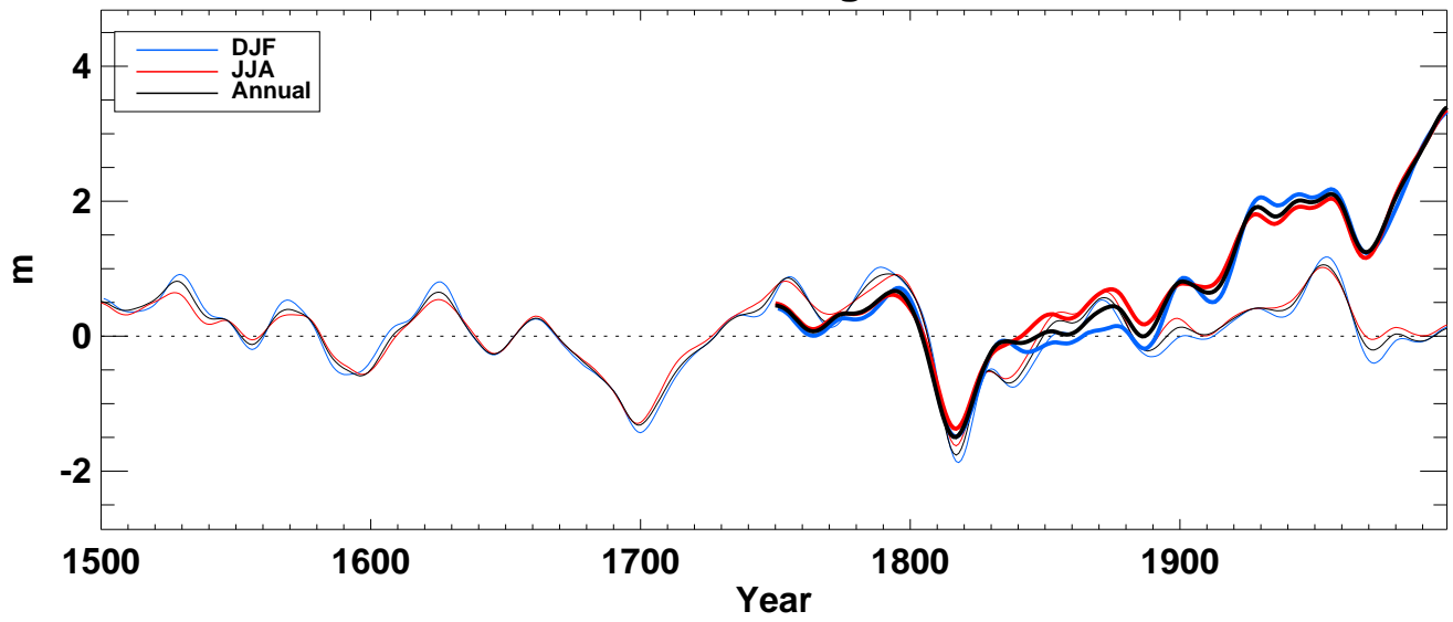
z850_ from hadcm3 averaged over Global full
