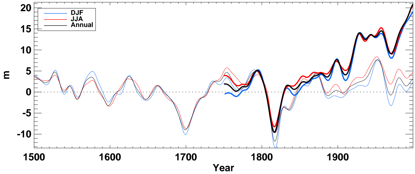
z500_ from hadcm3 averaged over Tropics ocean
