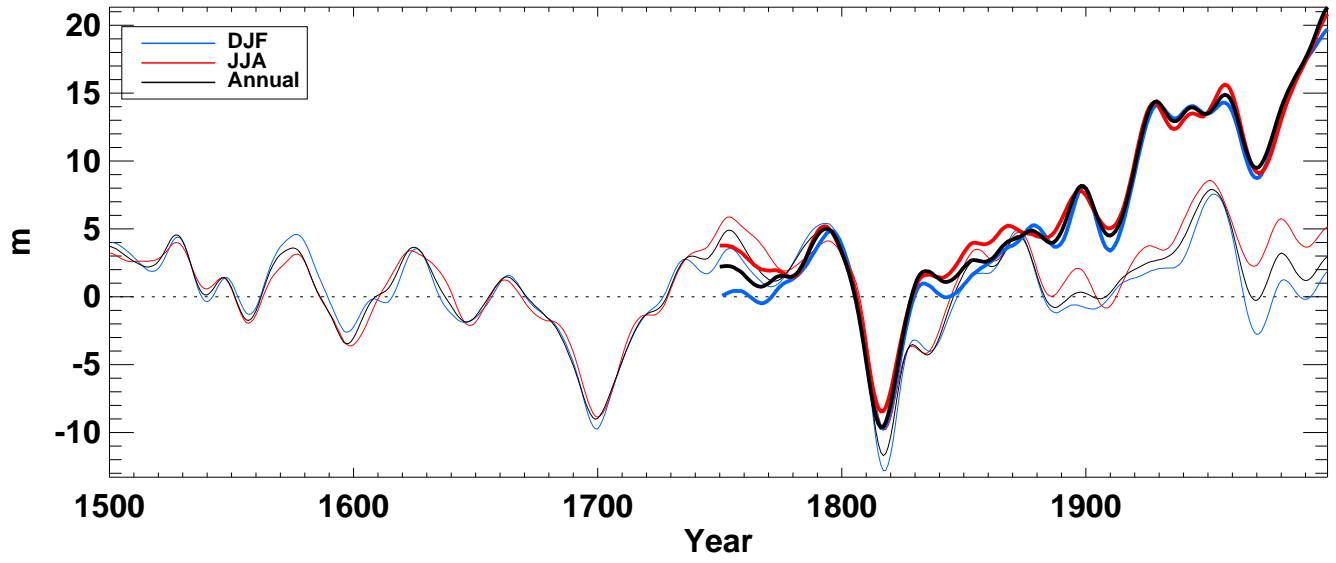
z500_ from hadcm3 averaged over Tropics land
