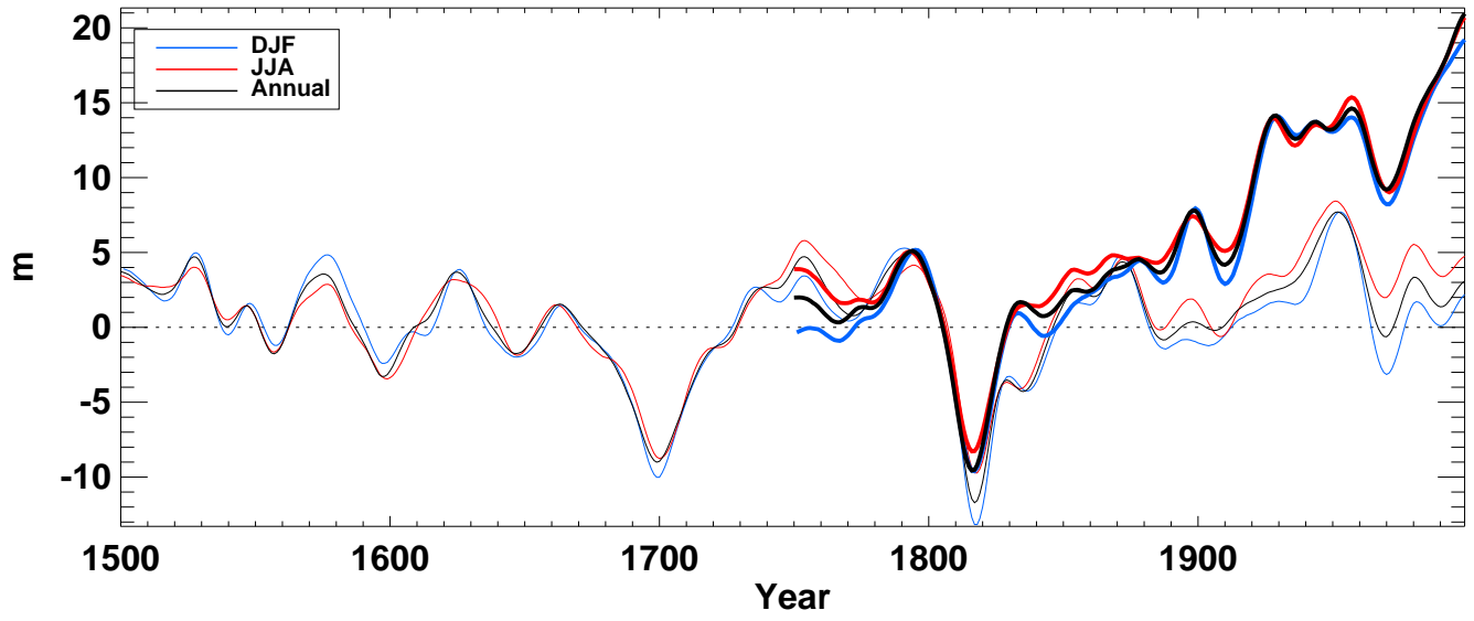
z500_ from hadcm3 averaged over Tropics full
