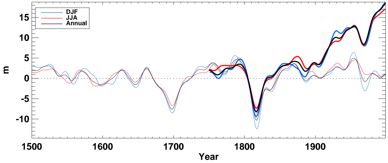
z500_ from hadcm3 averaged over SH ocean
