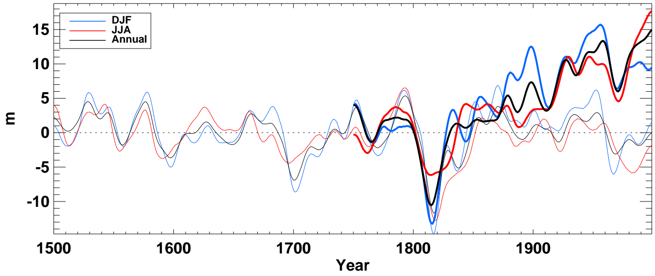
z500_ from hadcm3 averaged over SH land
