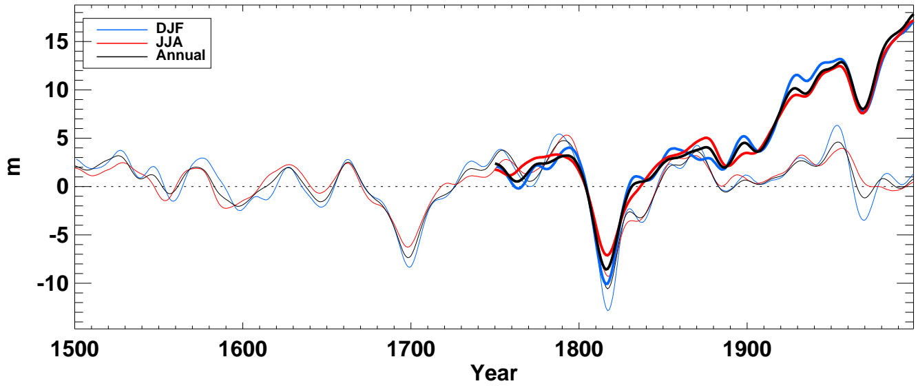
z500_ from hadcm3 averaged over SH full
