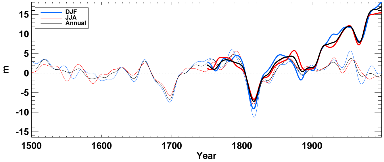
z500_ from hadcm3 averaged over S-extratropics ocean
