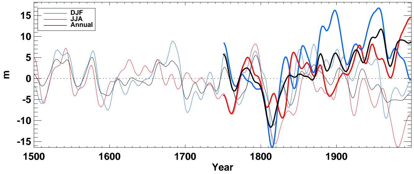
z500_ from hadcm3 averaged over S-extratropics land
