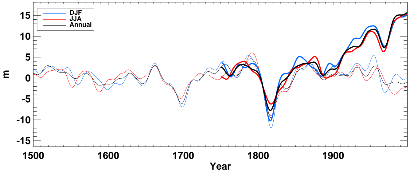
z500_ from hadcm3 averaged over S-extratropics full
