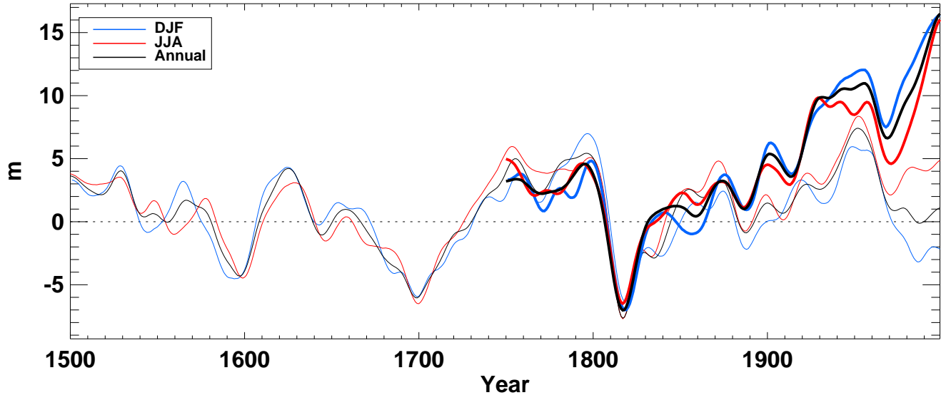
z500_ from hadcm3 averaged over NH ocean
