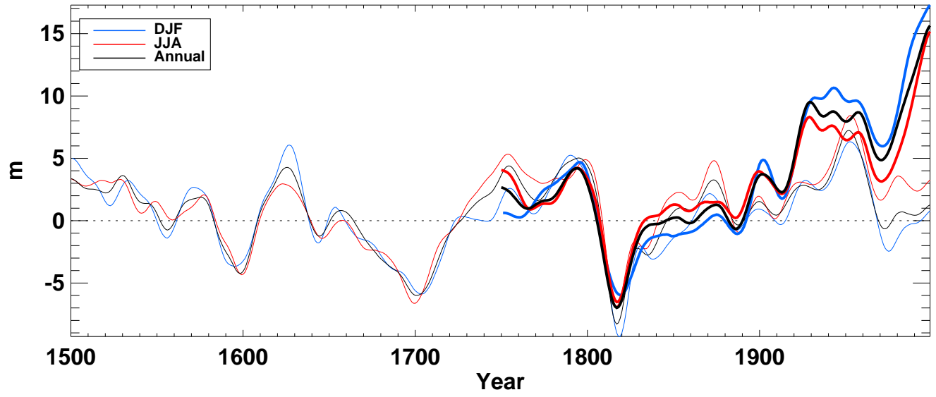
z500_ from hadcm3 averaged over NH land
