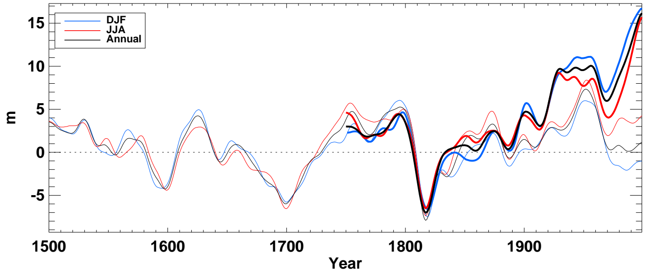
z500_ from hadcm3 averaged over NH full
