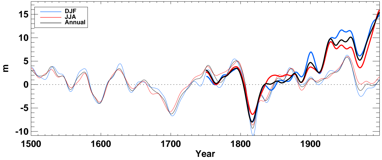
z500_ from hadcm3 averaged over Global land
