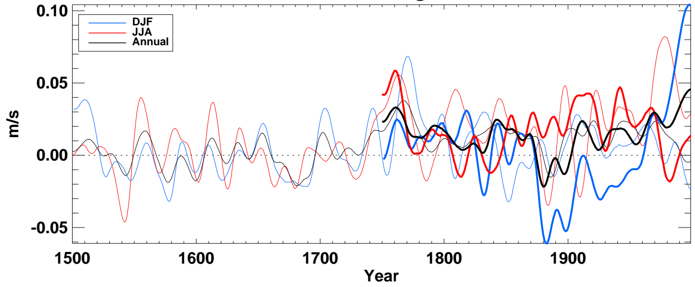
win10 from hadcm3 averaged over SH ocean
