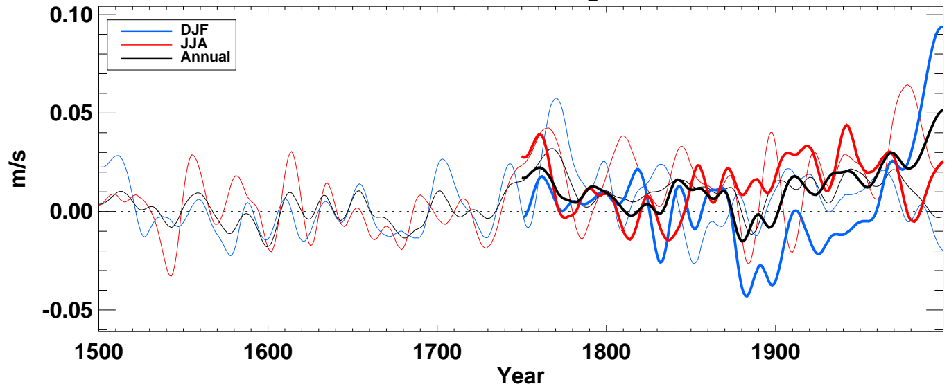
win10 from hadcm3 averaged over SH full
