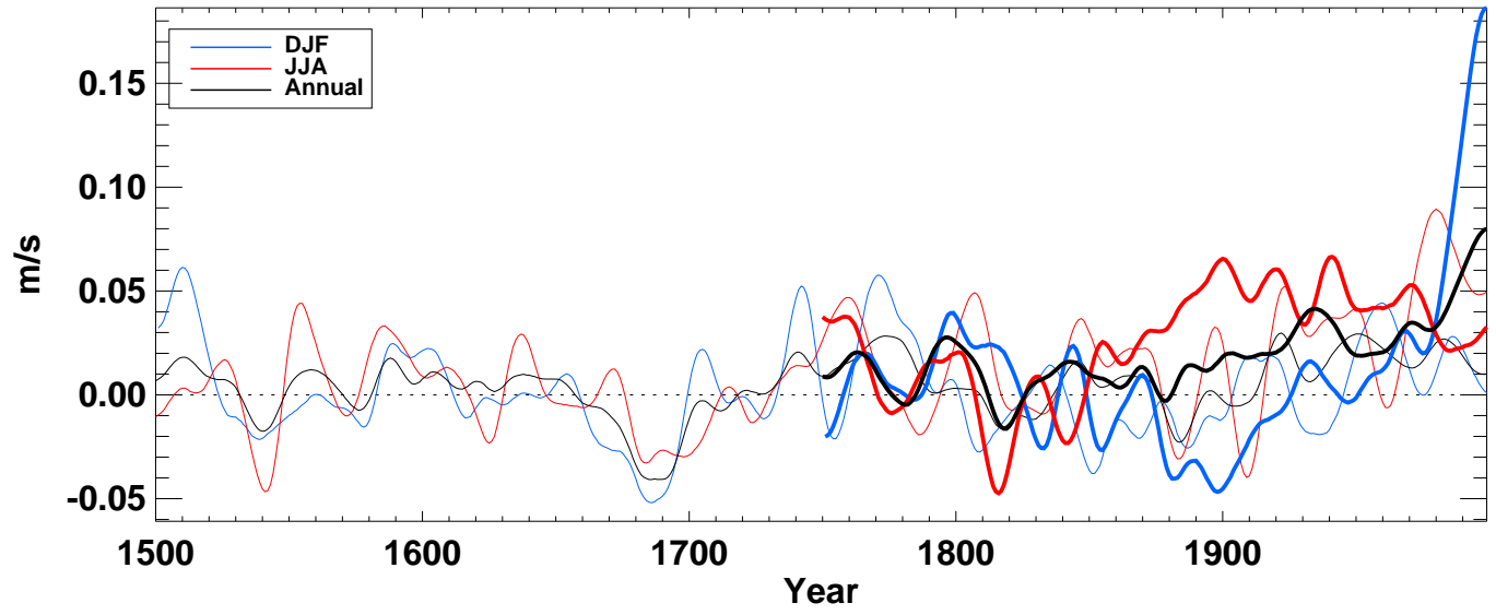
win10 from hadcm3 averaged over S-extratropics ocean
