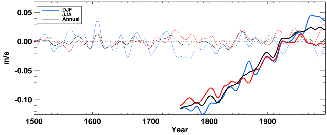
win10 from hadcm3 averaged over NH land
