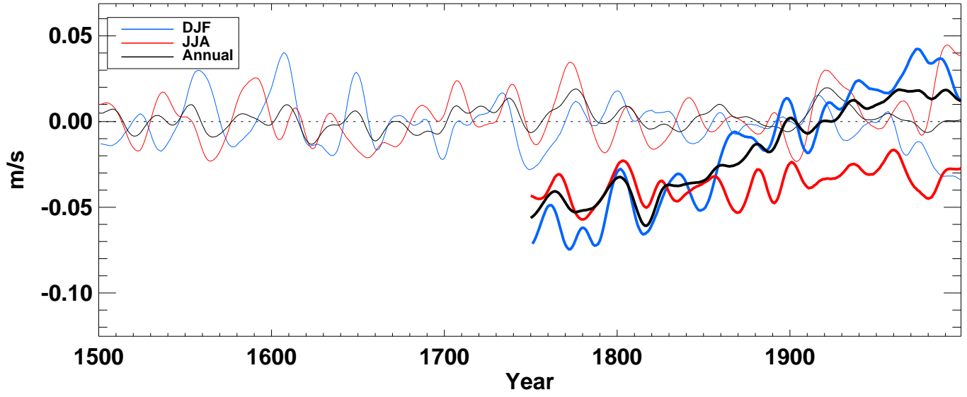
win10 from hadcm3 averaged over NH full
