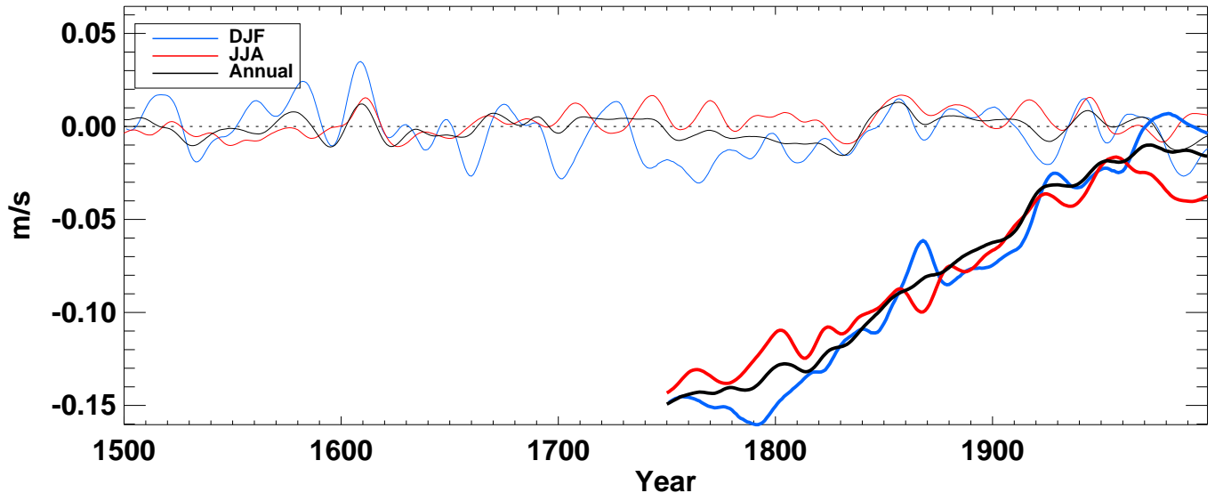
win10 from hadcm3 averaged over N-extratropics land
