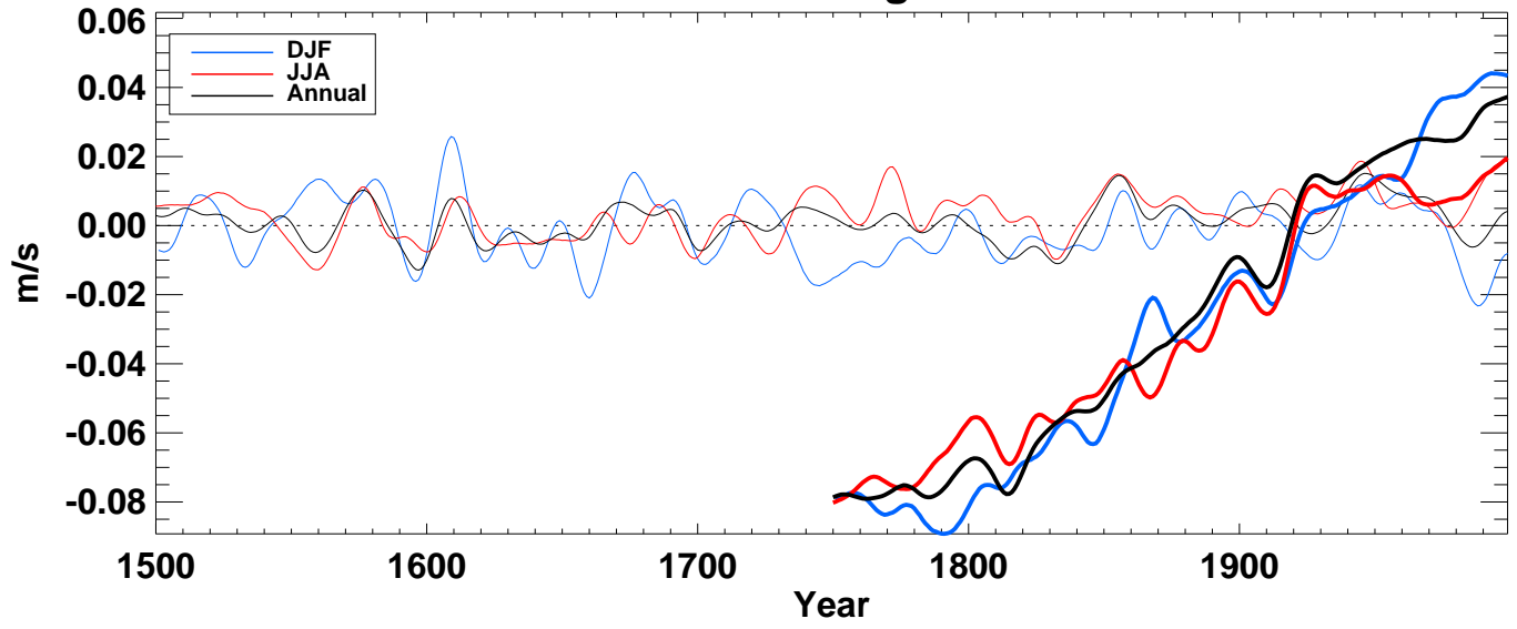
win10 from hadcm3 averaged over Global land
