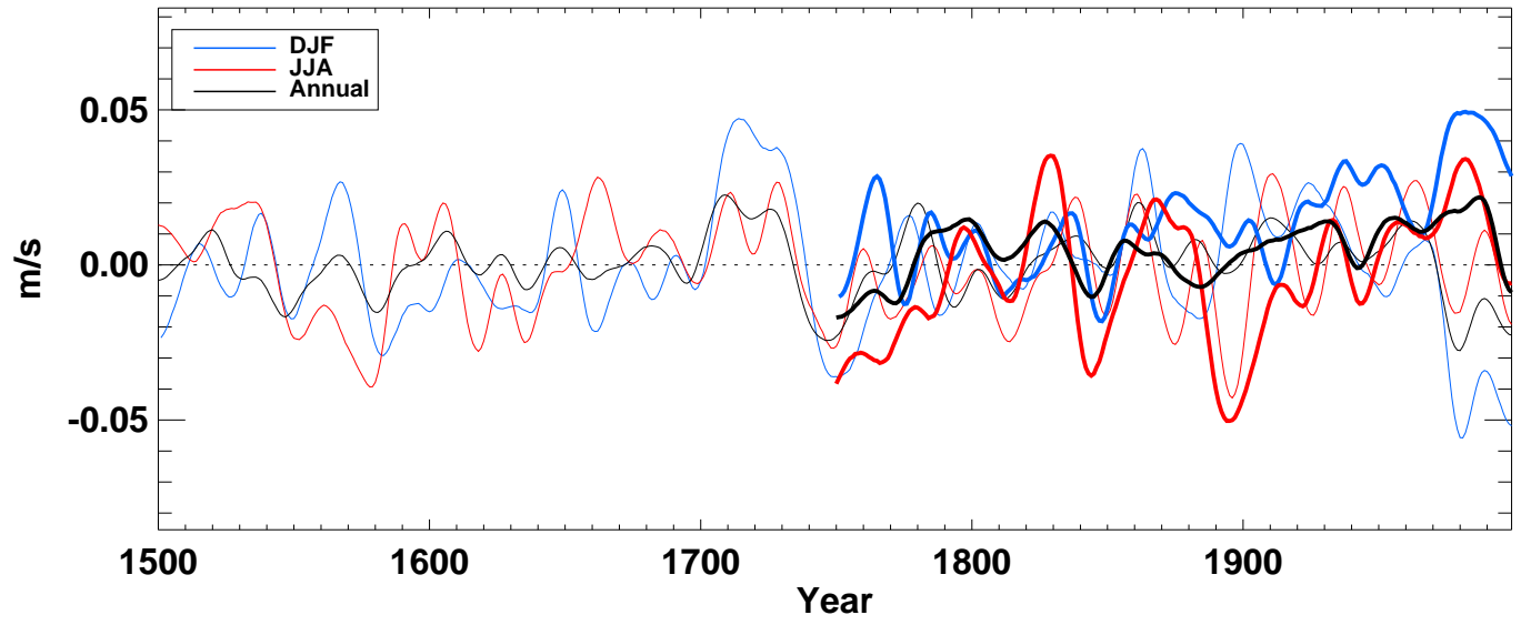
v500_ from hadcm3 averaged over Tropics ocean
