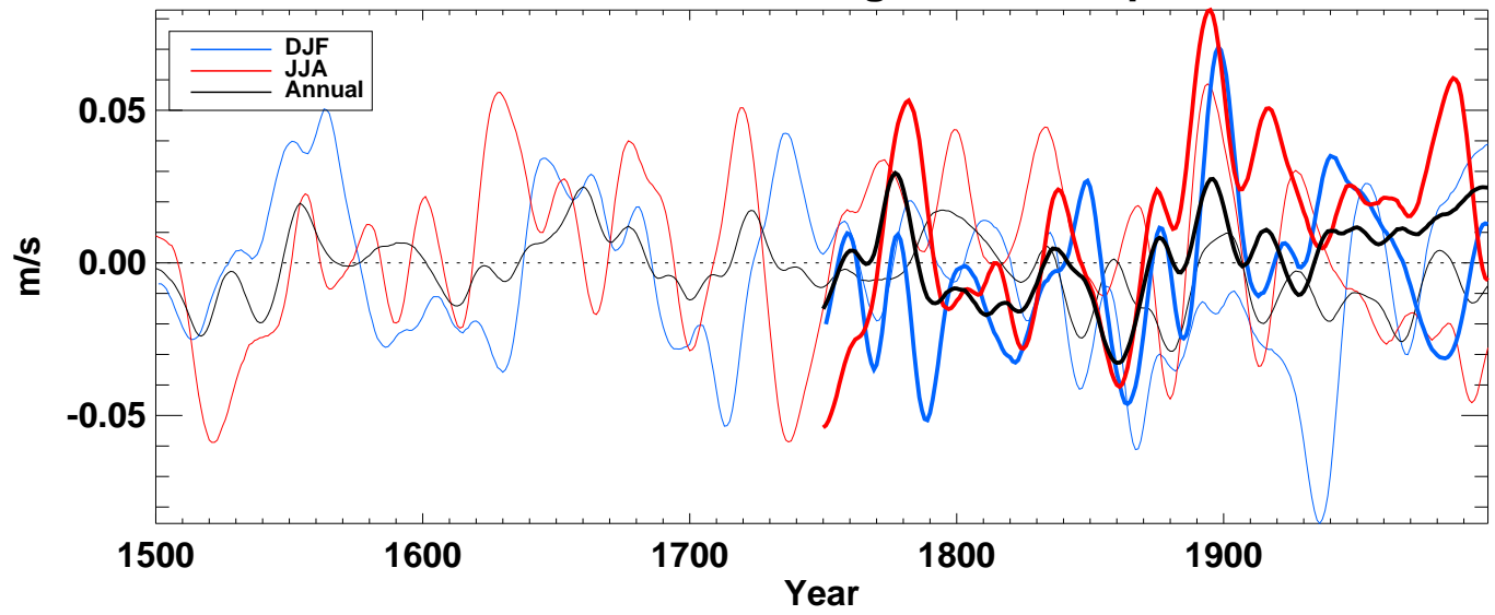
v500_ from hadcm3 averaged over Tropics land
