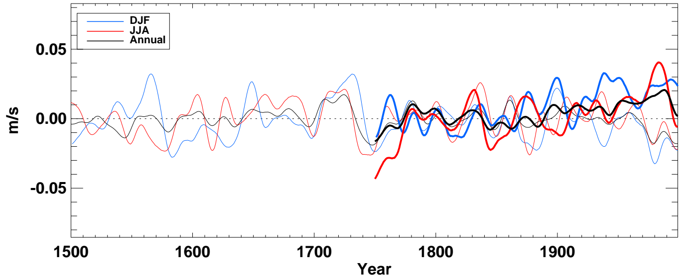
v500_ from hadcm3 averaged over Tropics full
