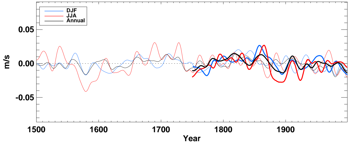
v500_ from hadcm3 averaged over SH ocean
