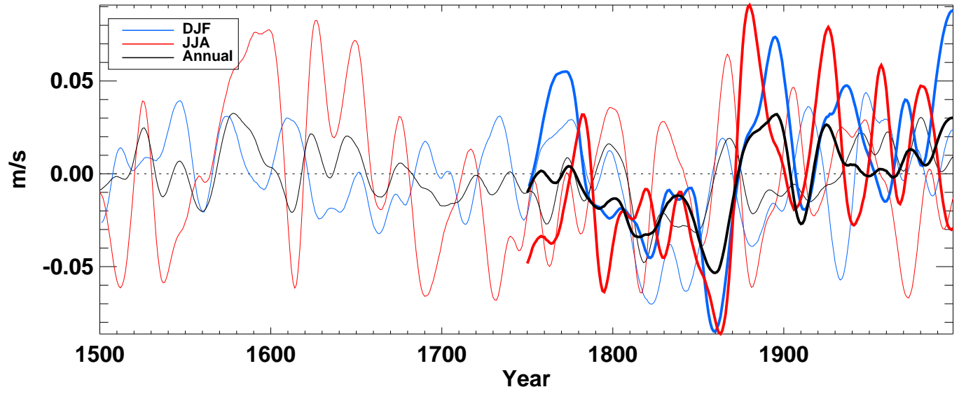
v500_ from hadcm3 averaged over SH land
