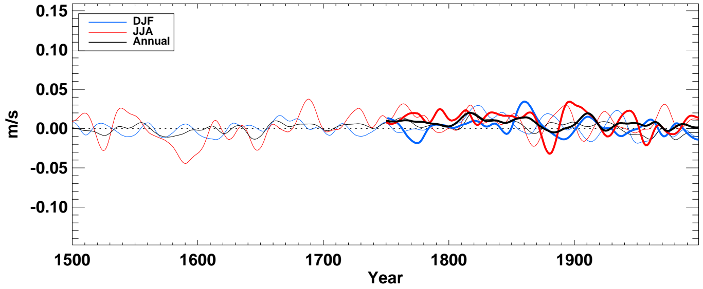
v500_ from hadcm3 averaged over S-extratropics ocean
