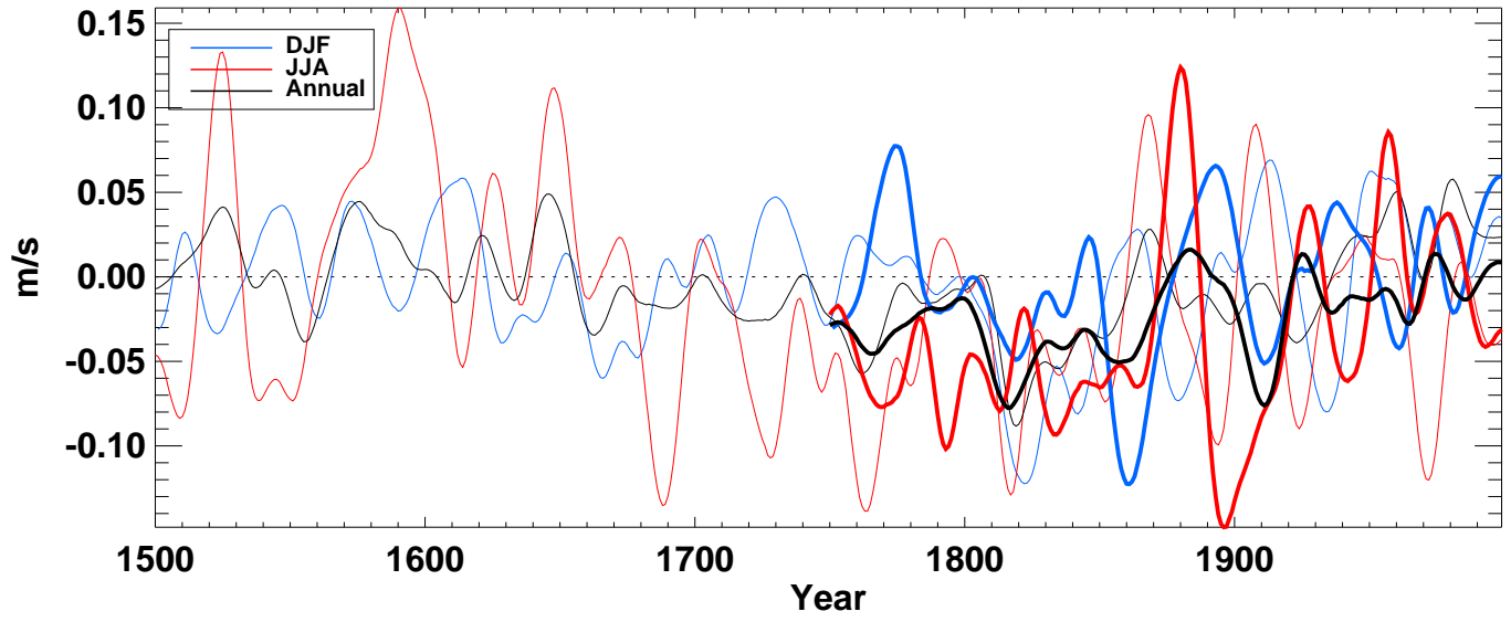
v500_ from hadcm3 averaged over S-extratropics land
