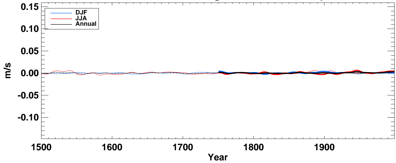
v500_ from hadcm3 averaged over S-extratropics full
