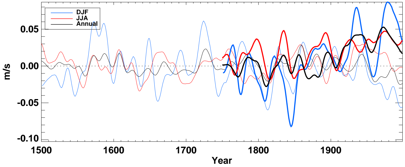
v500_ from hadcm3 averaged over NH ocean
