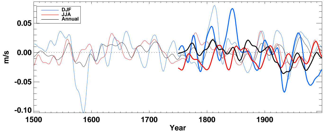
v500_ from hadcm3 averaged over NH land
