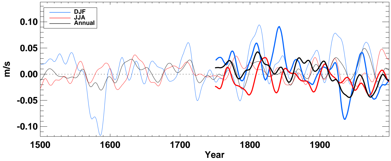
v500_ from hadcm3 averaged over N-extratropics land
