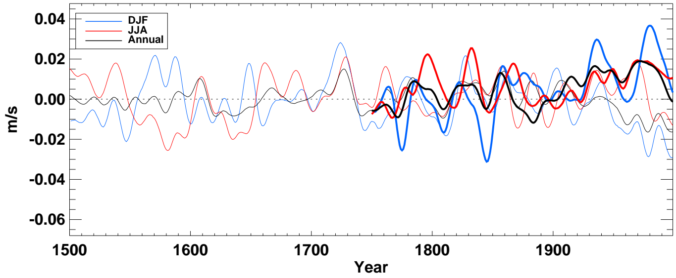
v500_ from hadcm3 averaged over Global ocean
