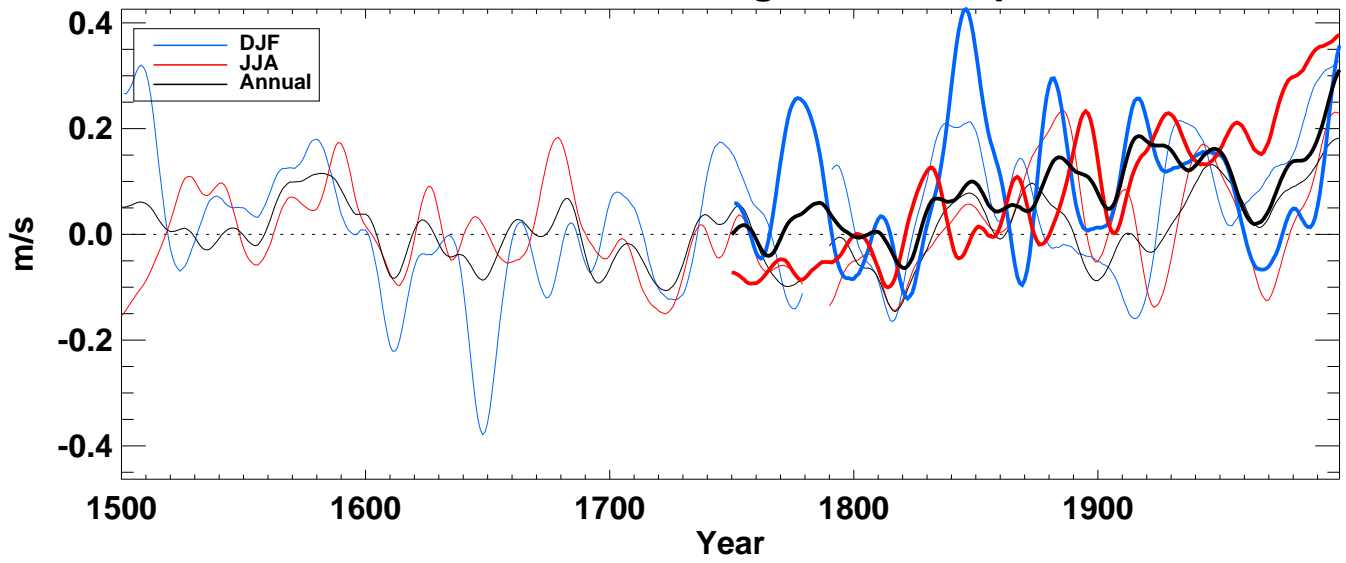
u500_ from hadcm3 averaged over Tropics ocean
