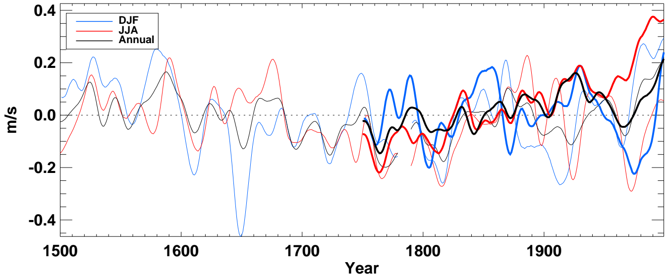
u500_ from hadcm3 averaged over Tropics land
