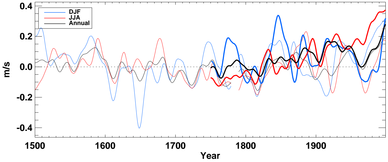
u500_ from hadcm3 averaged over Tropics full
