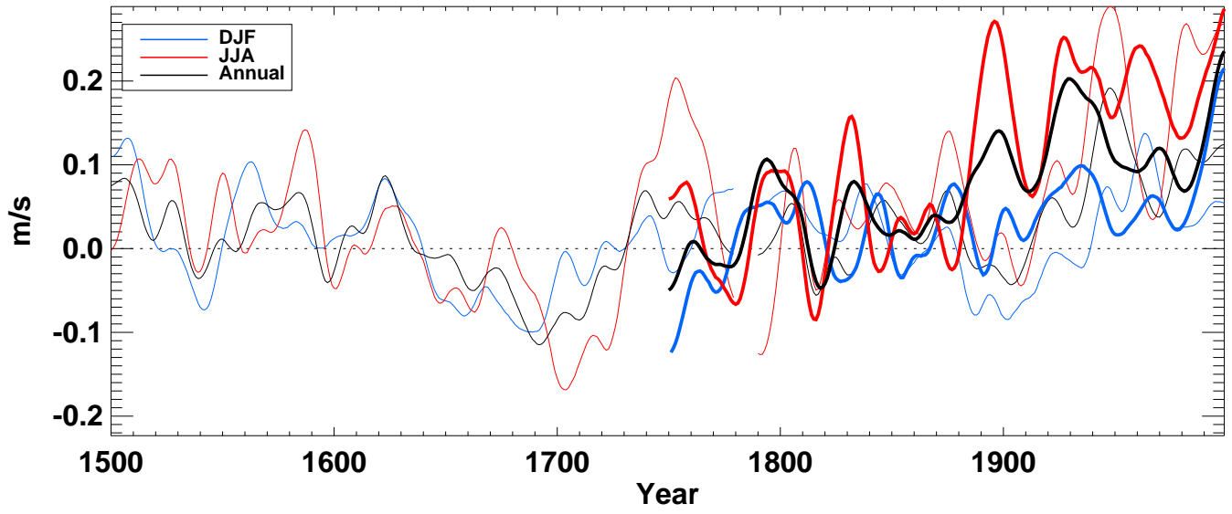
u500_ from hadcm3 averaged over SH ocean
