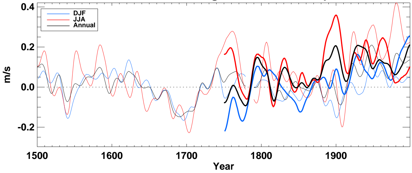
u500_ from hadcm3 averaged over S-extratropics ocean
