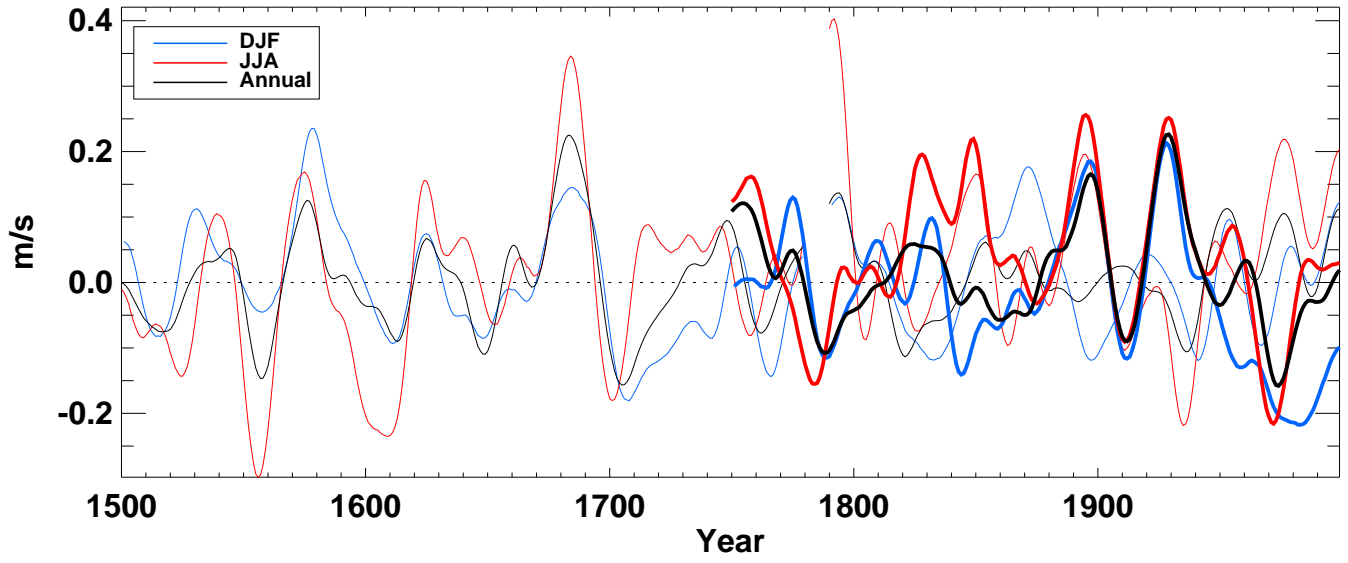
u500_ from hadcm3 averaged over S-extratropics land
