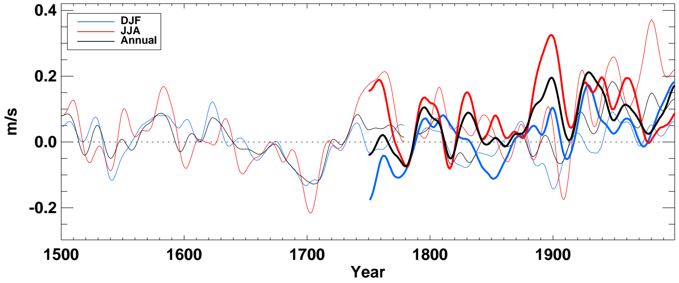
u500_ from hadcm3 averaged over S-extratropics full
