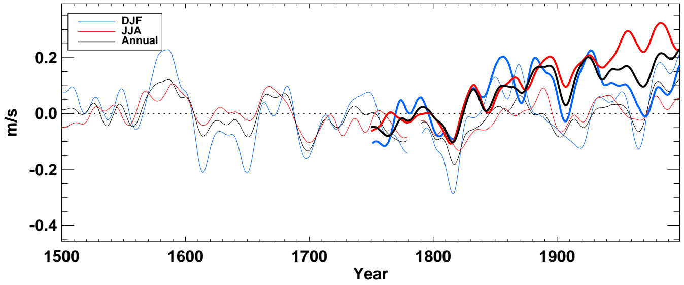
u500_ from hadcm3 averaged over NH full
