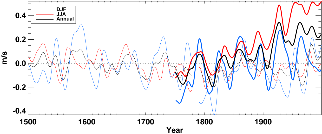
u500_ from hadcm3 averaged over N-extratropics ocean
