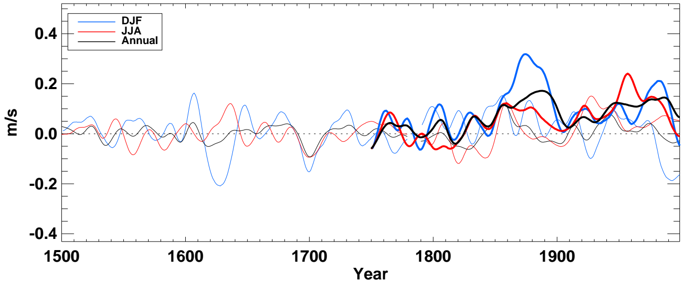
u500_ from hadcm3 averaged over N-extratropics land
