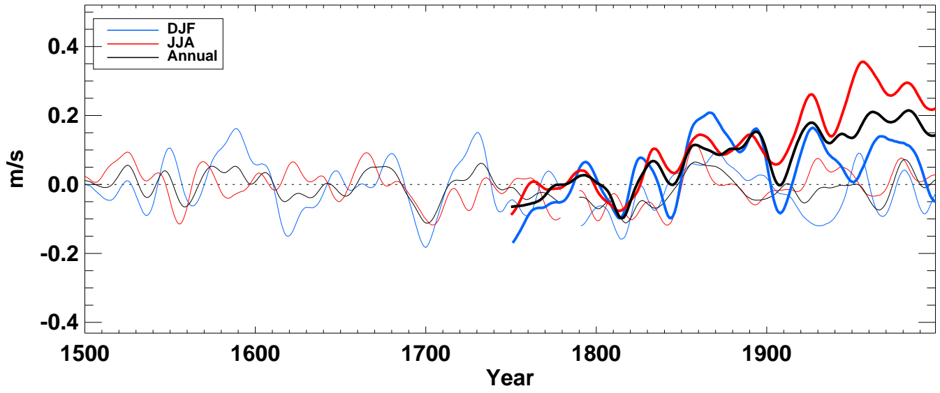
u500_ from hadcm3 averaged over N-extratropics full
