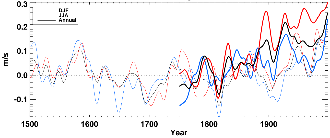
u500_ from hadcm3 averaged over Global ocean
