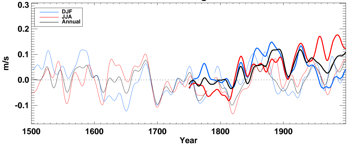
u500_ from hadcm3 averaged over Global land
