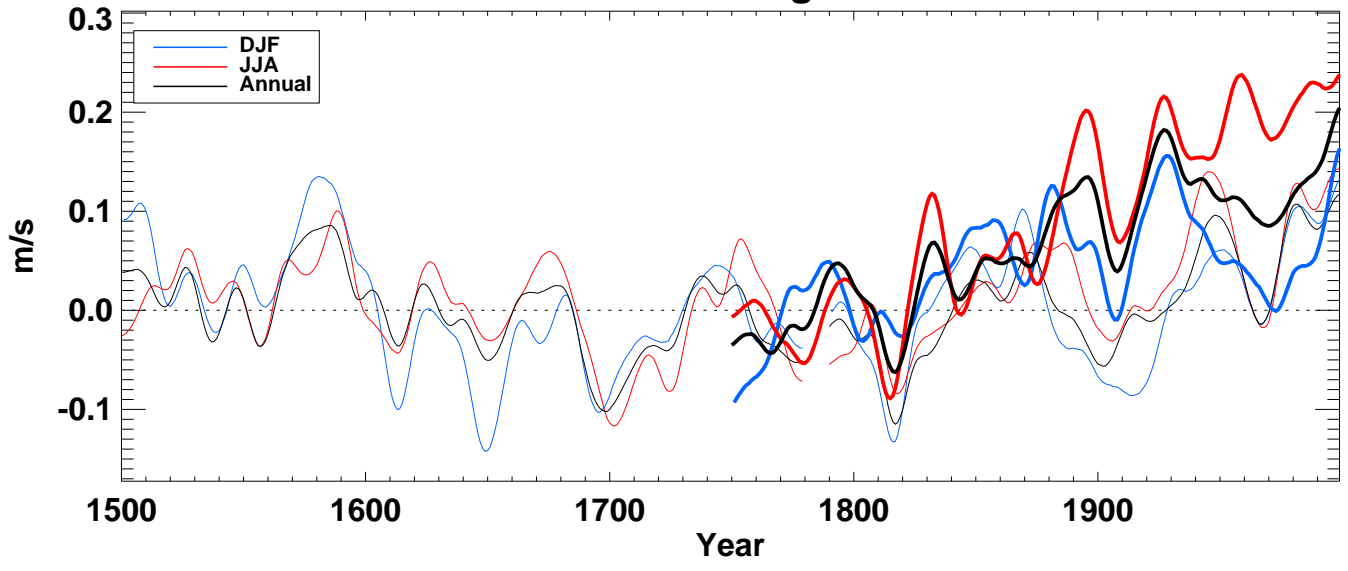
u500_ from hadcm3 averaged over Global full
