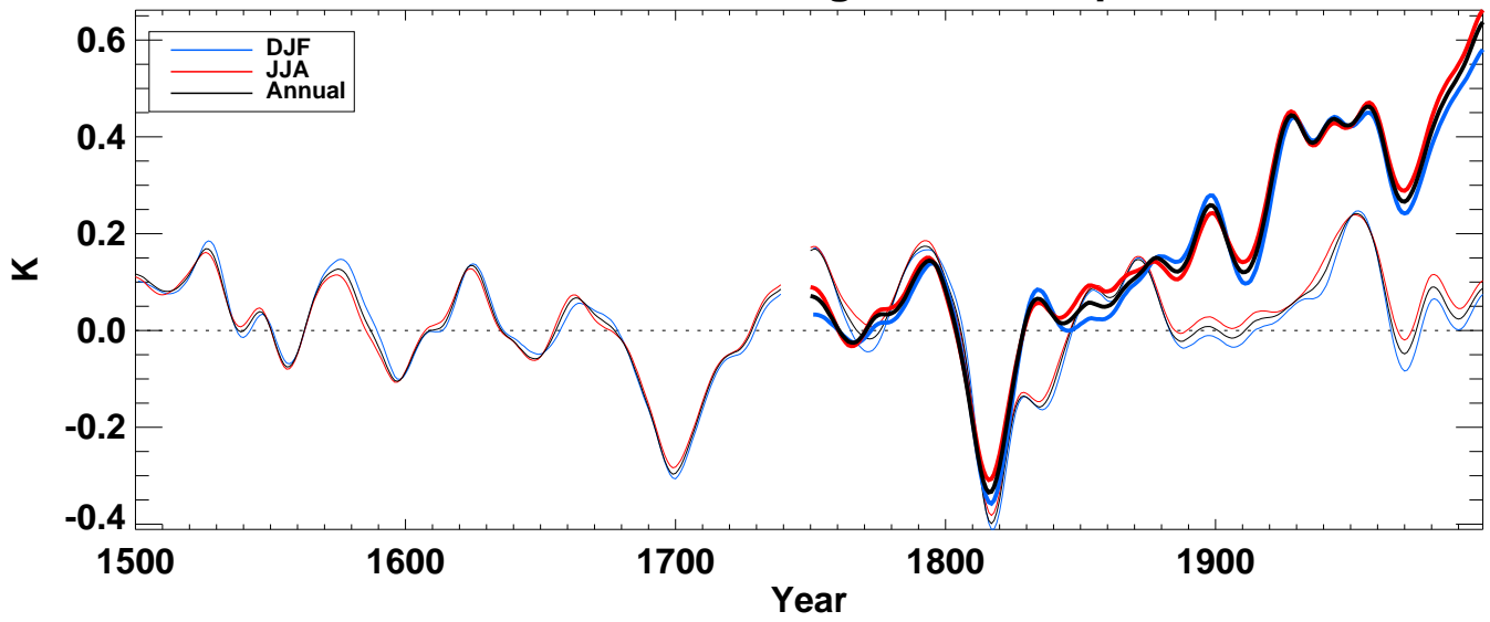
sst__ from hadcm3 averaged over Tropics ocean
