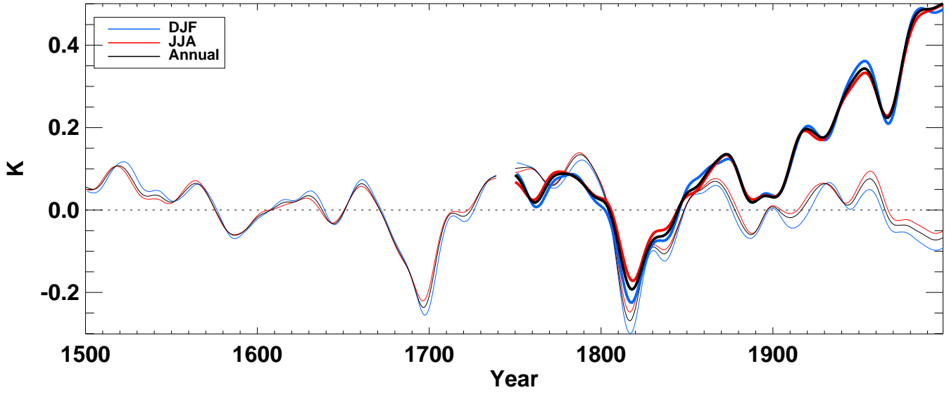
sst__ from hadcm3 averaged over S-extratropics ocean
