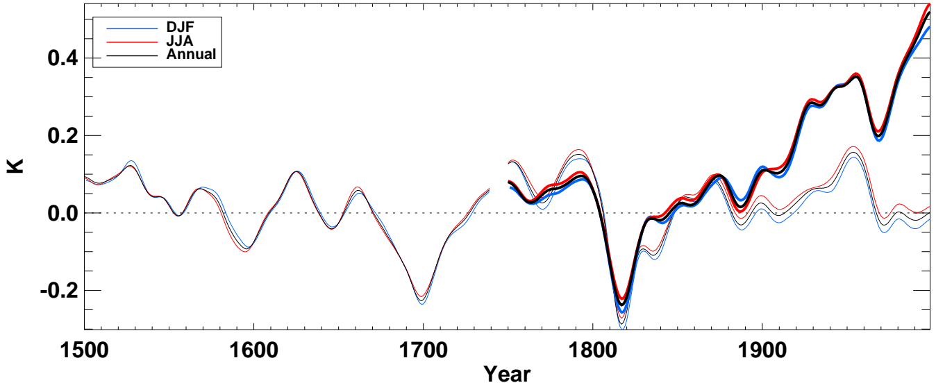
sst__ from hadcm3 averaged over Global ocean
